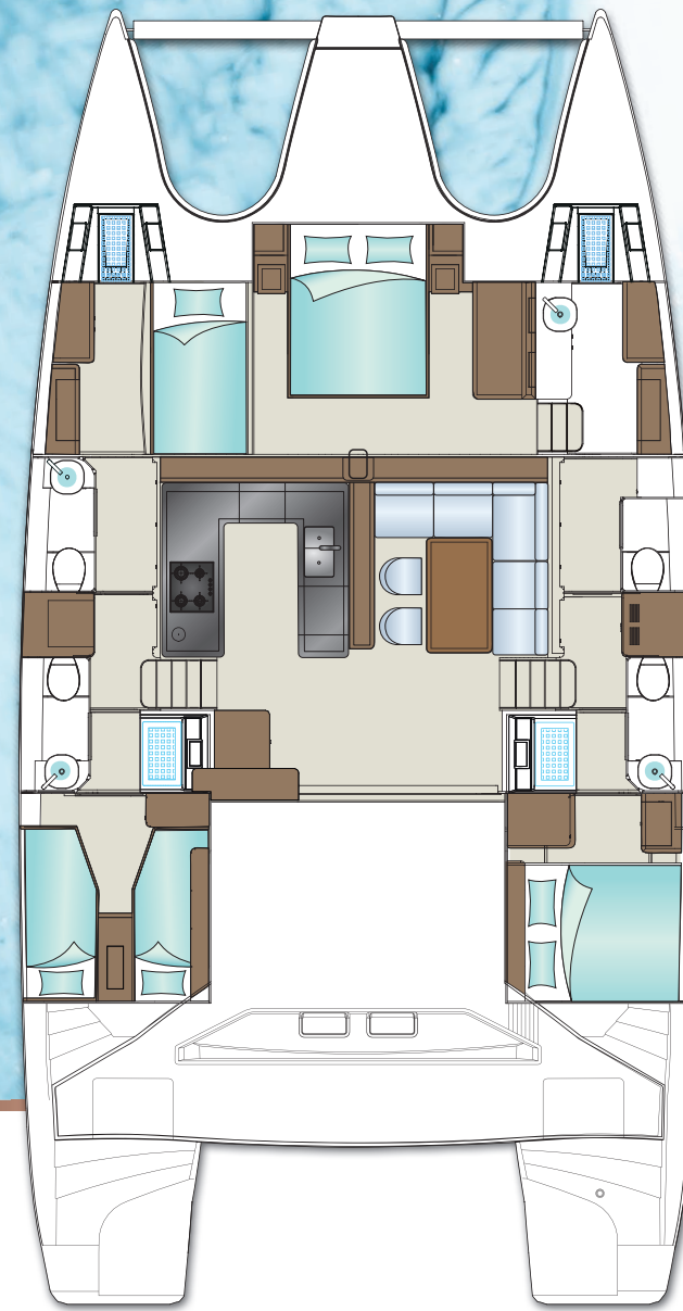
LOWER DECK Option 4 cabins 2/3 – 1/3
